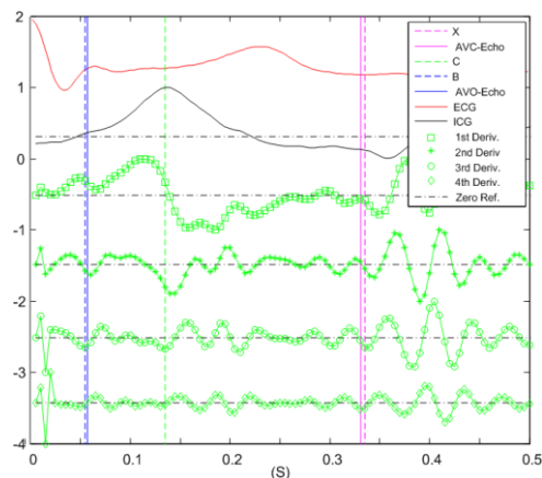
Fig. 5: Illustration of B and X point detection method using high-order derivatives in an ICG signal with a subtle B-point notch. AVO-Echo and AVC-Echo define, respectively, the detected aortic valve opening and closing moments using echocardiography. Dashed vertical markers define B, X and C points detected using the
