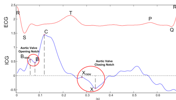
Fig. 1: Definition of characteristic points for aortic valve events in the Impedance Cardiogram. Points B and X are the traditional definitions for opening and closing events of the aortic valve. B_{new} and X_{new} correspond to the
